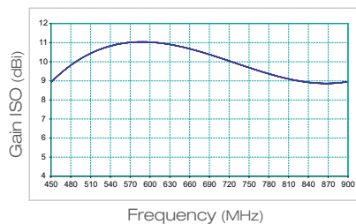
LP45HV - UHF Band
