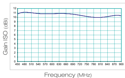
LP45F - UHF Band
