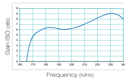
LPV345F - Band III
