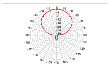
LP34F - Band III
