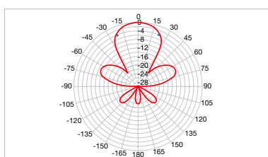
LPV345F - UHF Band
