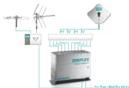
SIG9708CI - Using a msw to distribute signals to all receivers
