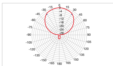
LP345F - UHF Band
