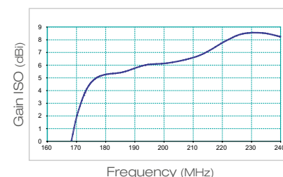
LP345MF - Band III
