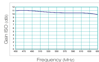
LP34F - Band IV
