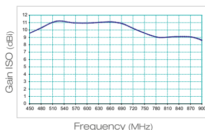
LP345F - UHF Band
