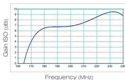
LP34F - Band III
