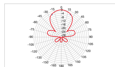
LPV345F - Band III
