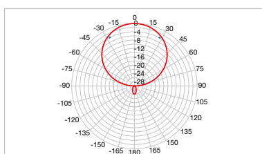
LP45F - UHF Band
