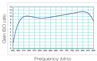
LPV345F - UHF Band
