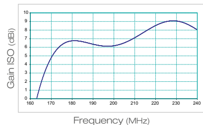
LPV345HV - Band III
