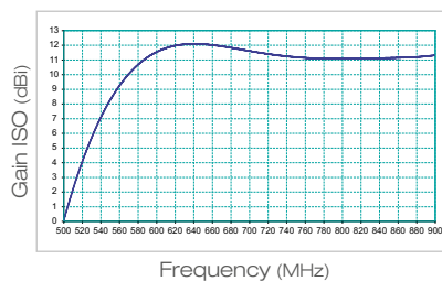
LP5F - Band V
